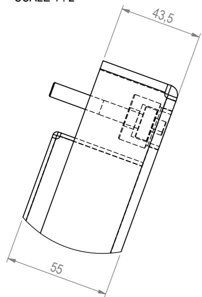
DETAIL A SCALE 1 : 2
