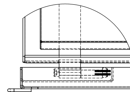
DETAIL C SCALE 1 : 5
